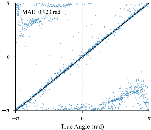
Elbow ( \theta_2 ) Linearity
