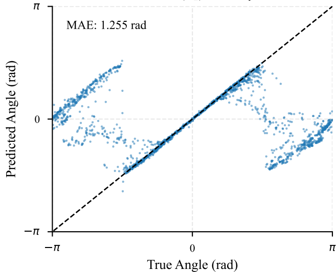
Shoulder ( \theta_1 ) Linearity
