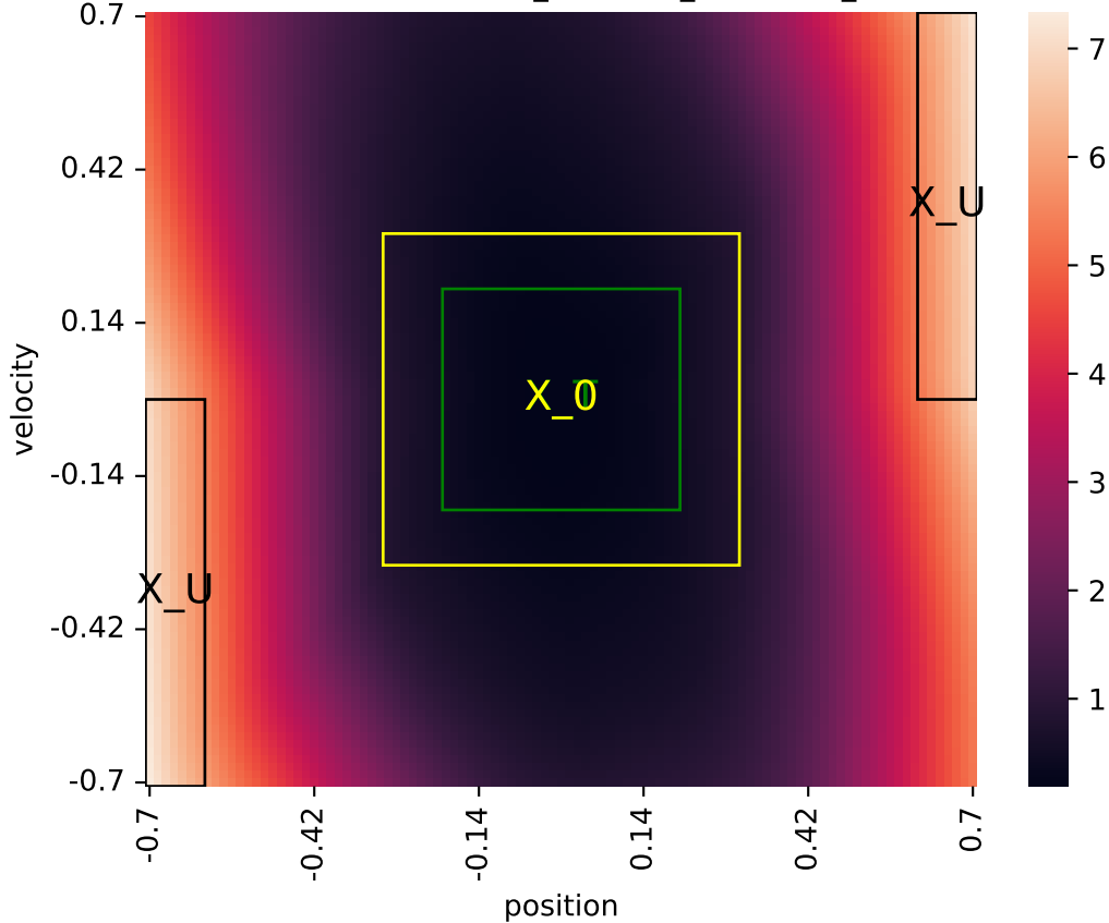
Learned certificate (2026-06-01_22-24-36_certificate_iteration=11)
