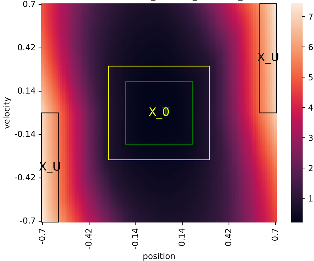
Learned certificate (2026-06-01_22-39-59_certificate_iteration=13)
