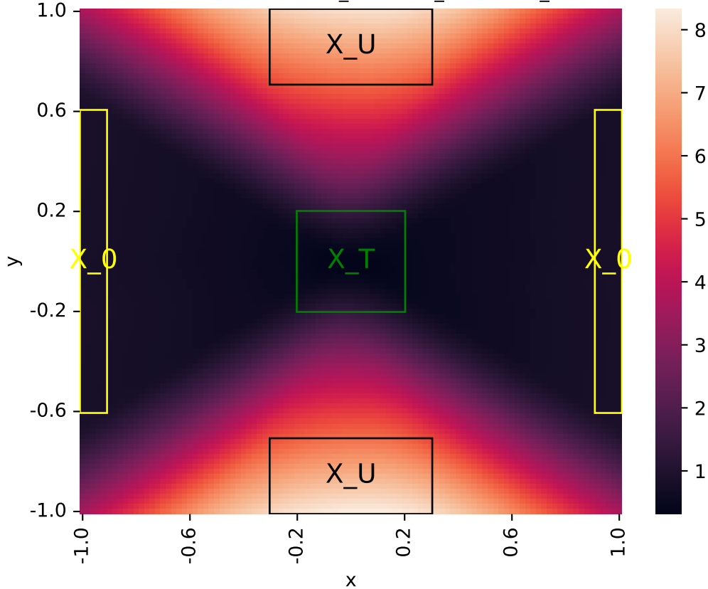
Learned certificate (2026-06-01_23-24-53_certificate_iteration=4)
