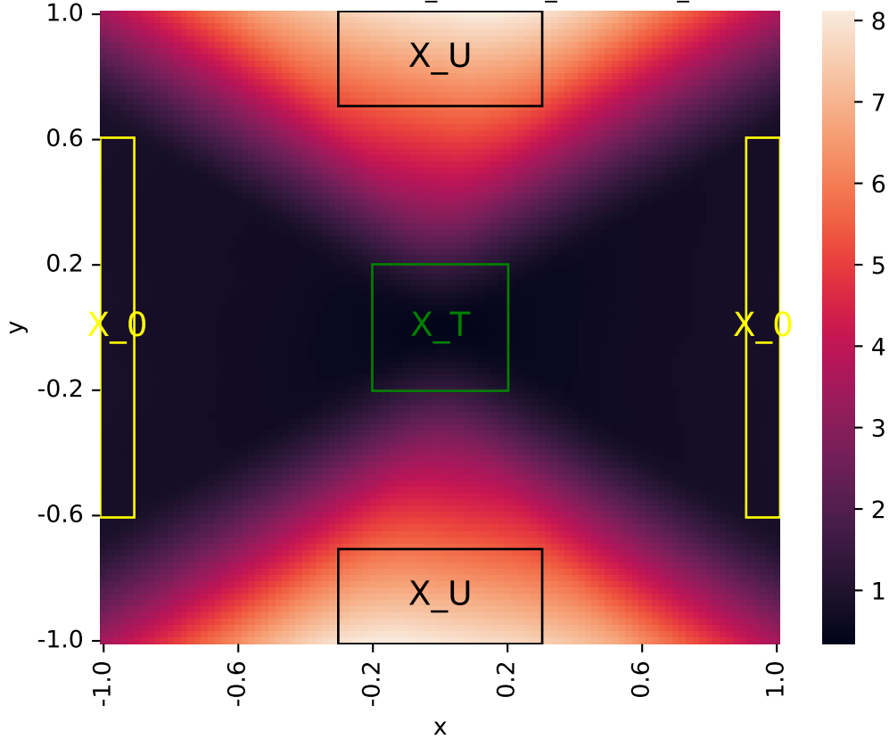
Learned certificate (2026-06-01_23-36-56_certificate_iteration=5)
