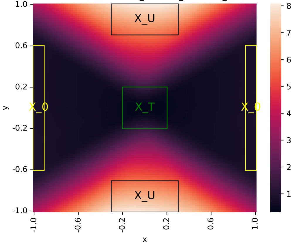
Learned certificate (2026-06-01_23-52-25_certificate_iteration=4)
