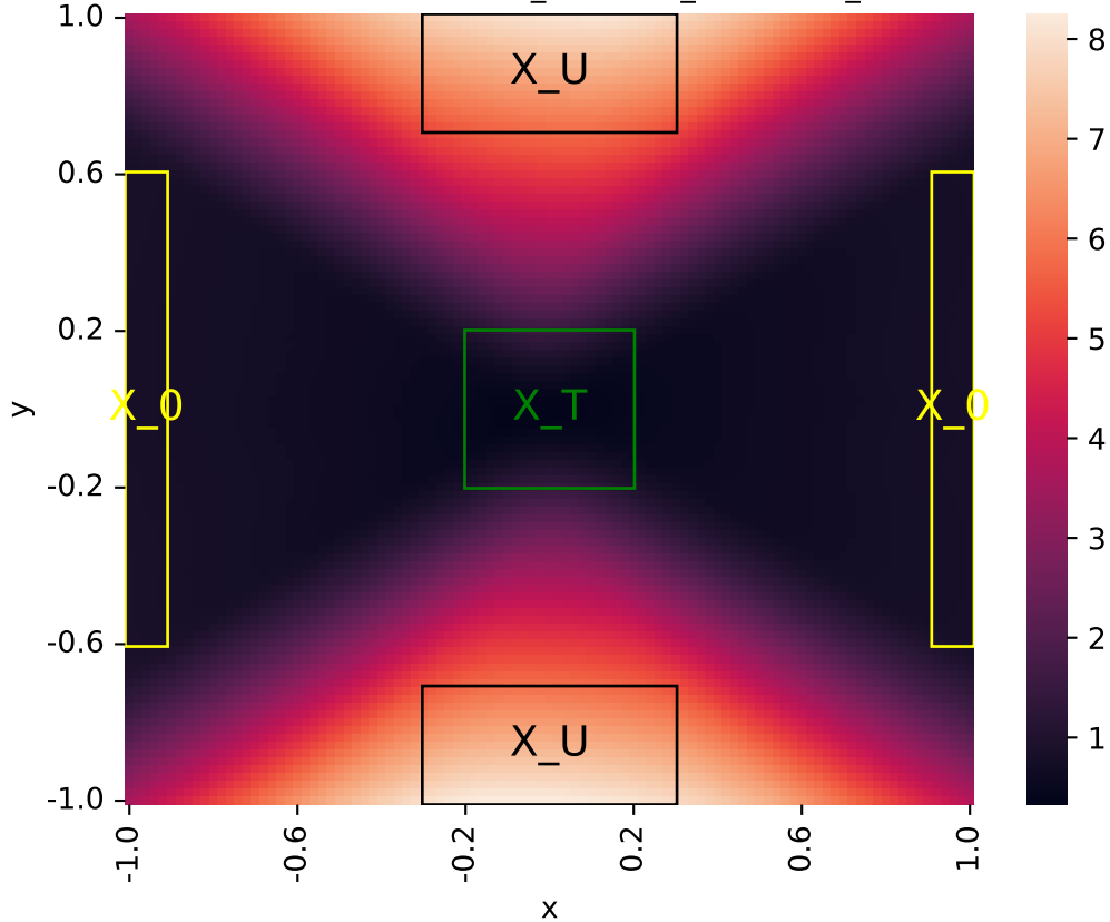
Learned certificate (2026-06-02_00-00-49_certificate_iteration=4)
