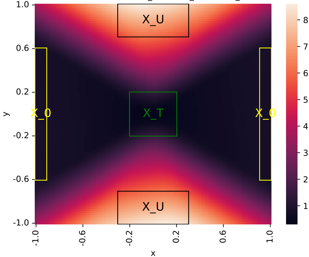
Learned certificate (2026-06-02_00-11-28_certificate_iteration=4)
