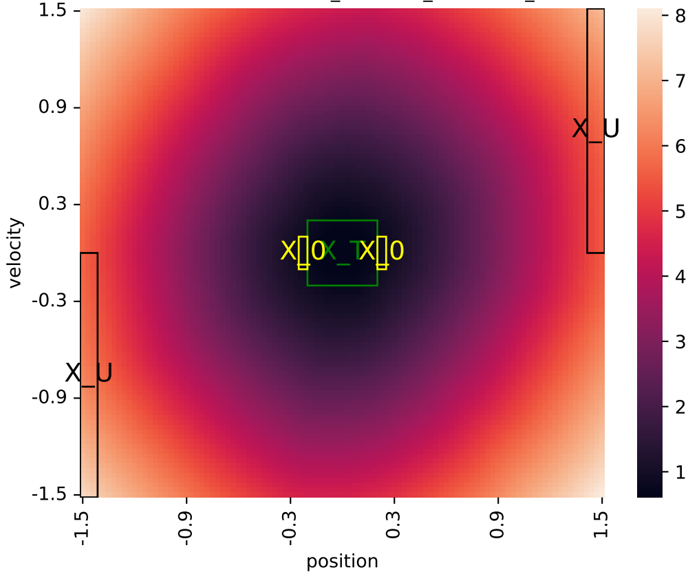
Learned certificate (2026-06-02_00-38-09_certificate_iteration=1)
