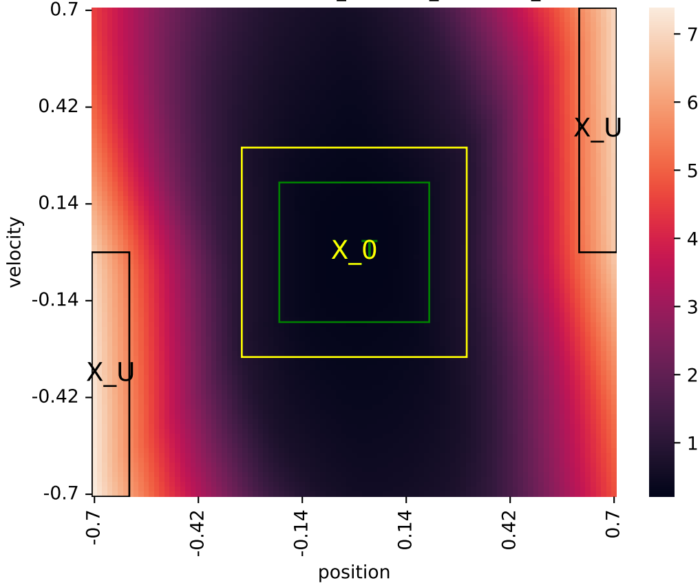
Learned certificate (2026-05-31_01-54-42_certificate_iteration=10)
