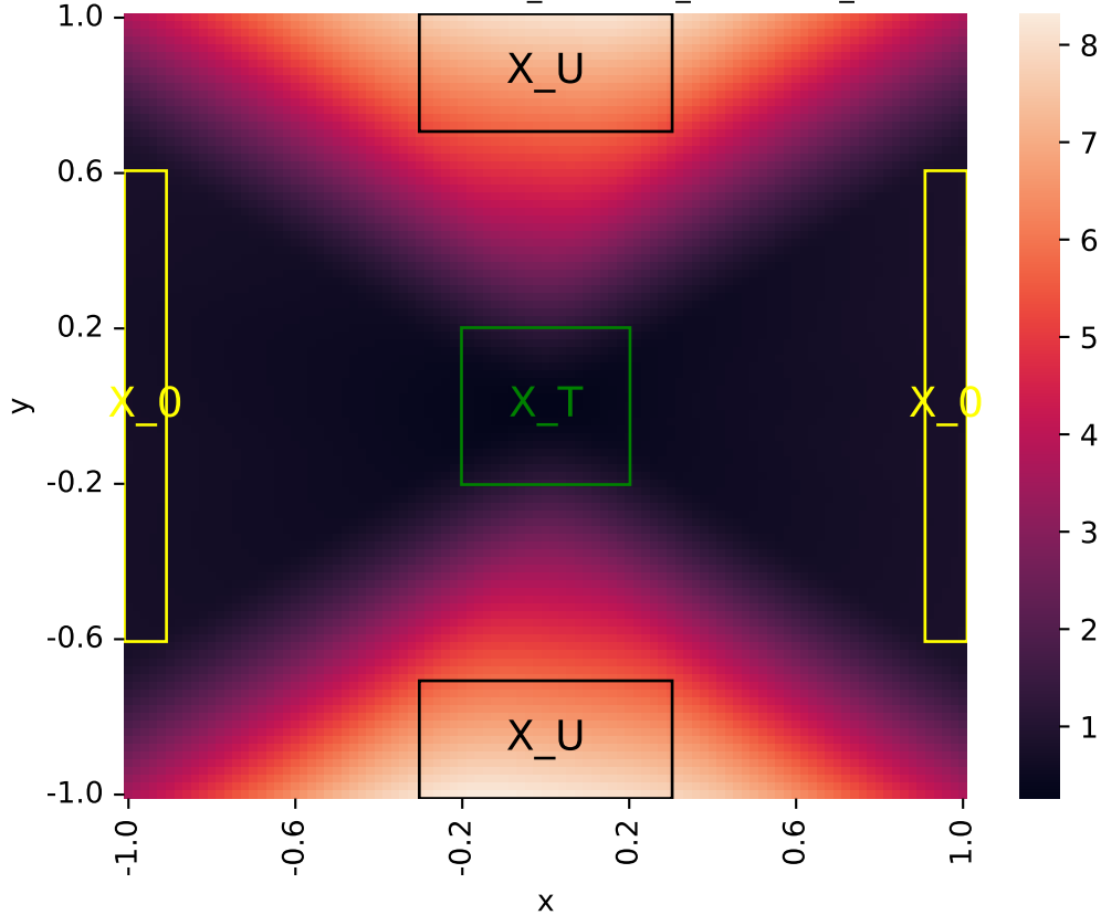
Learned certificate (2026-05-31_04-53-09_certificate_iteration=4)
