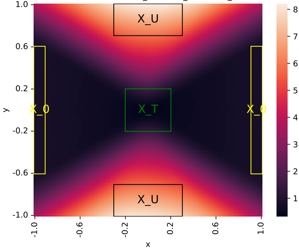
Learned certificate (2026-05-31_05-16-50_certificate_iteration=4)
