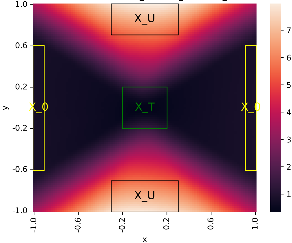
Learned certificate (2026-05-31_05-31-30_certificate_iteration=4)
