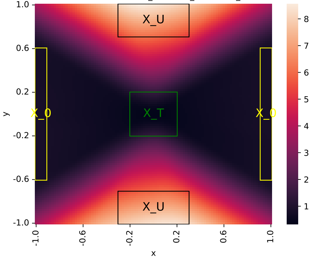
Learned certificate (2026-05-31_05-37-54_certificate_iteration=4)
