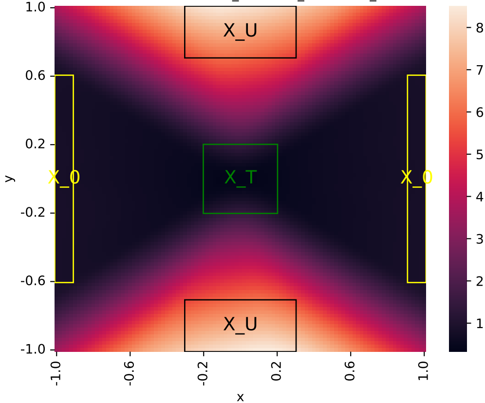
Learned certificate (2026-05-31_05-46-00_certificate_iteration=4)
