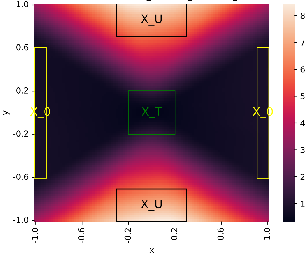
Learned certificate (2026-05-31_05-48-42_certificate_iteration=4)
