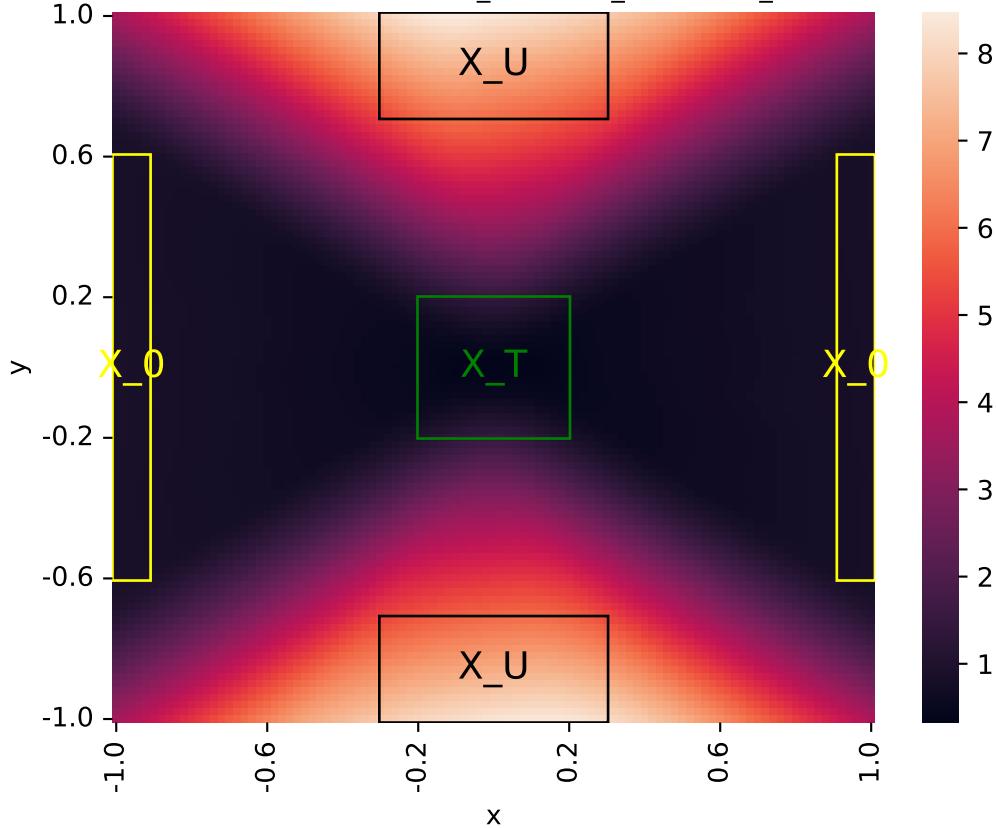
Learned certificate (2026-05-31_05-54-04_certificate_iteration=4)
