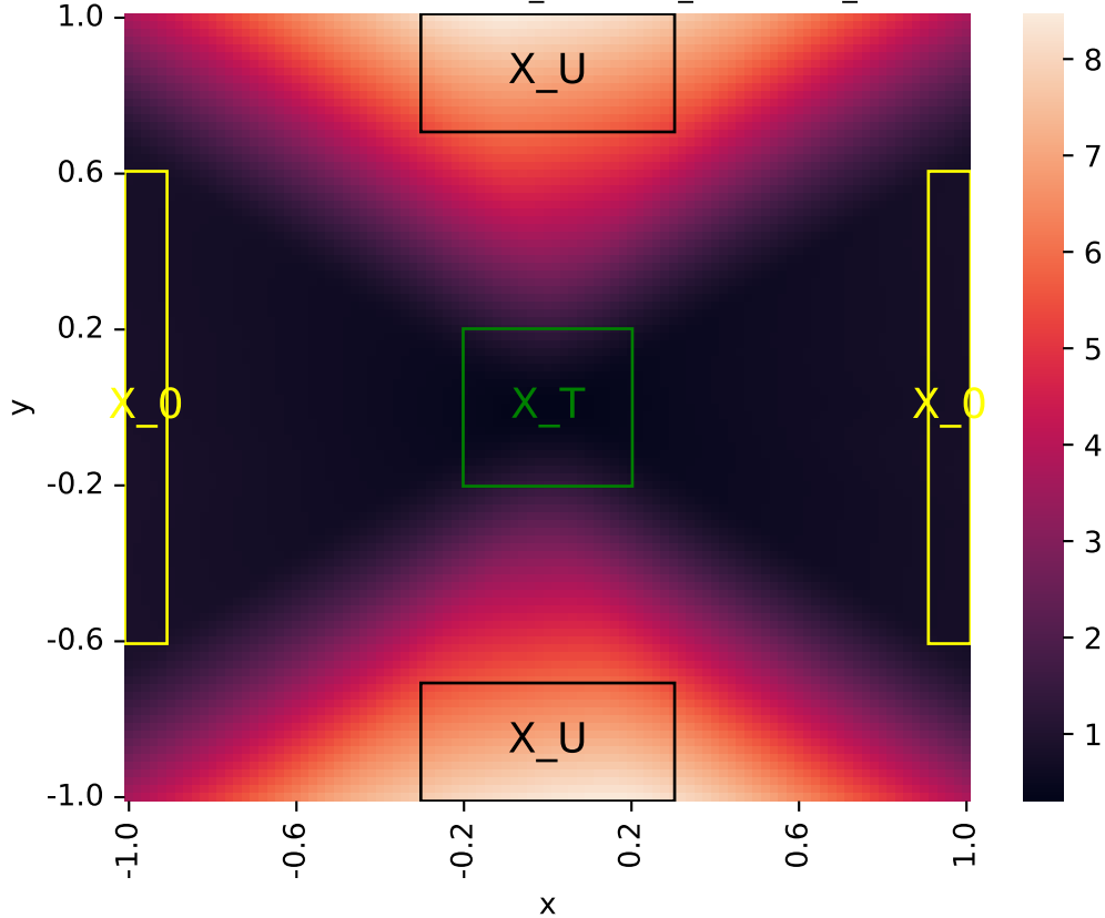
Learned certificate (2026-05-31_05-58-49_certificate_iteration=4)
