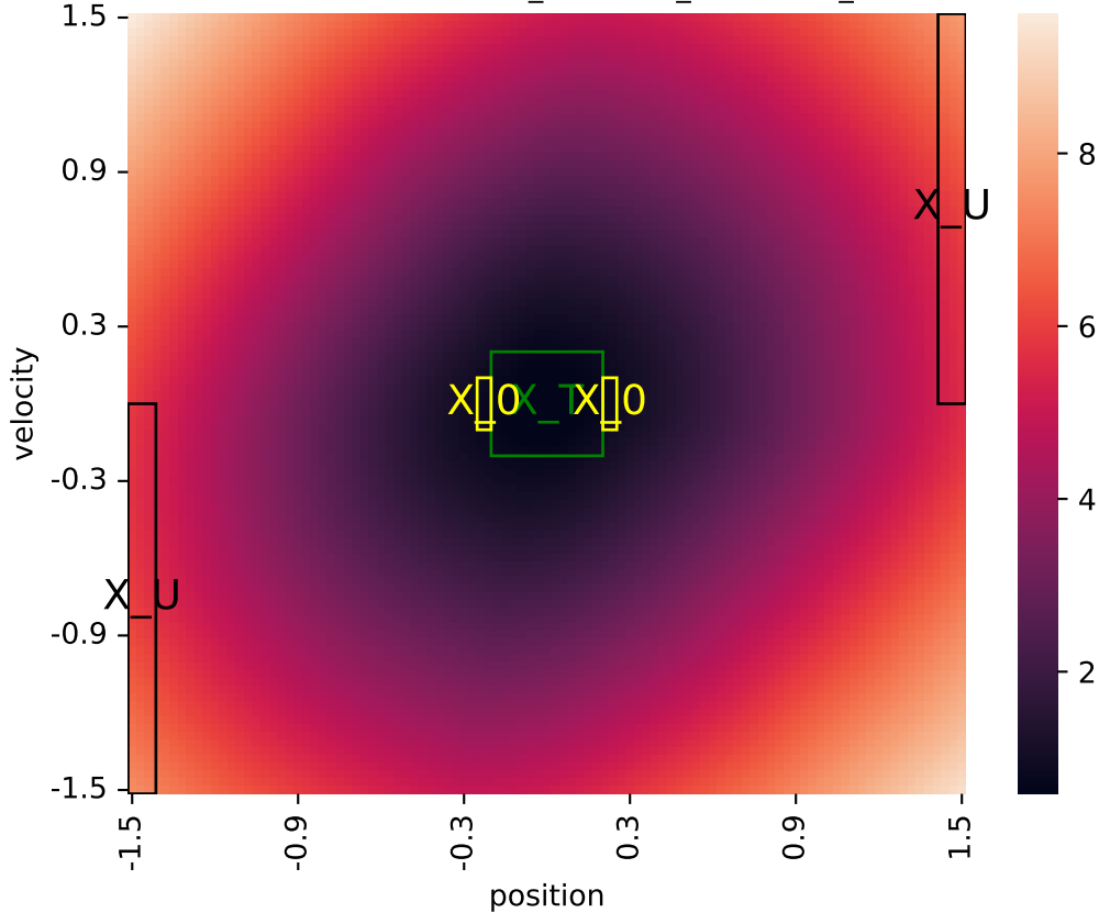
Learned certificate (2026-05-31_06-26-26_certificate_iteration=2)
