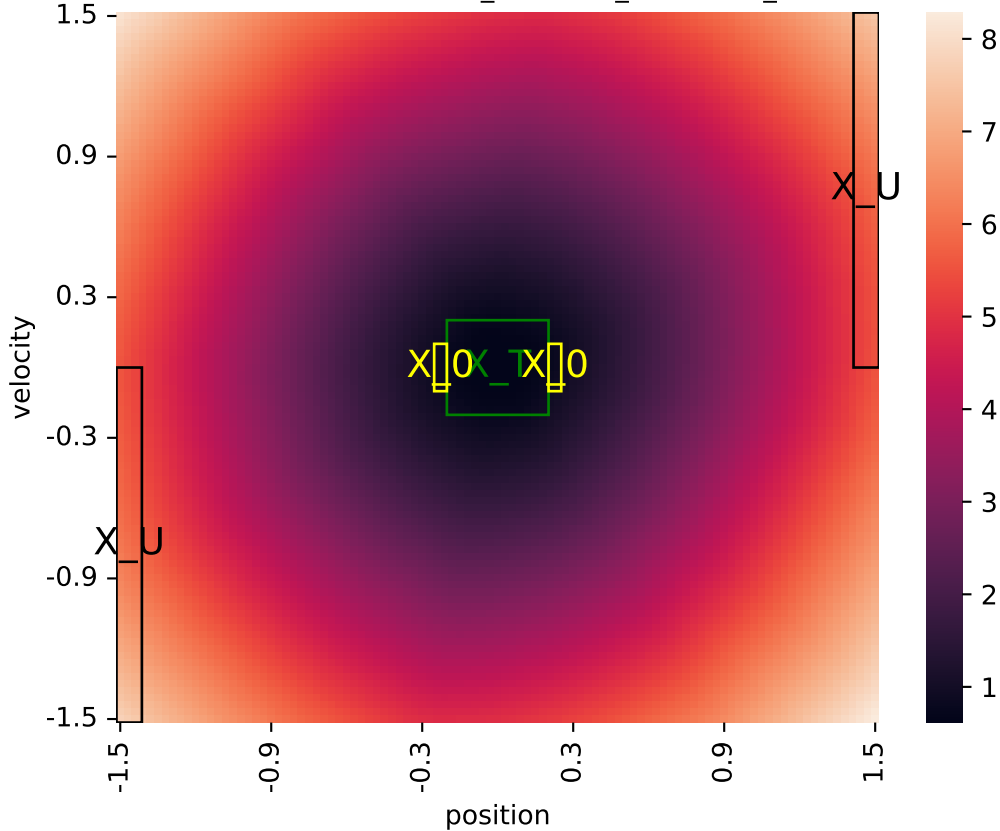
Learned certificate (2026-05-31_06-30-24_certificate_iteration=1)
