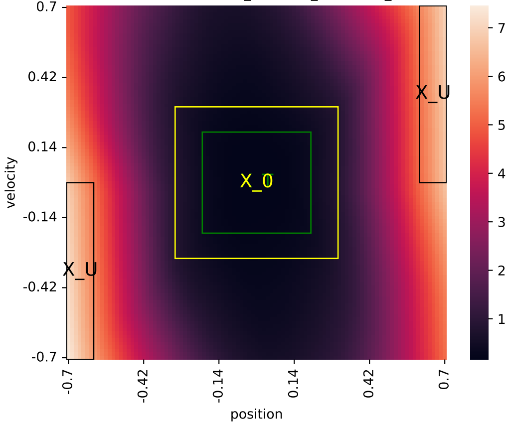
Learned certificate (2026-06-02_18-53-14_certificate_iteration=10)
