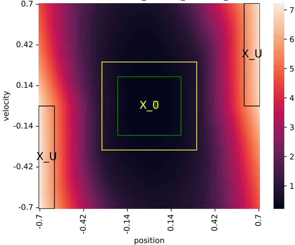
Learned certificate (2026-06-02_19-25-04_certificate_iteration=11)
