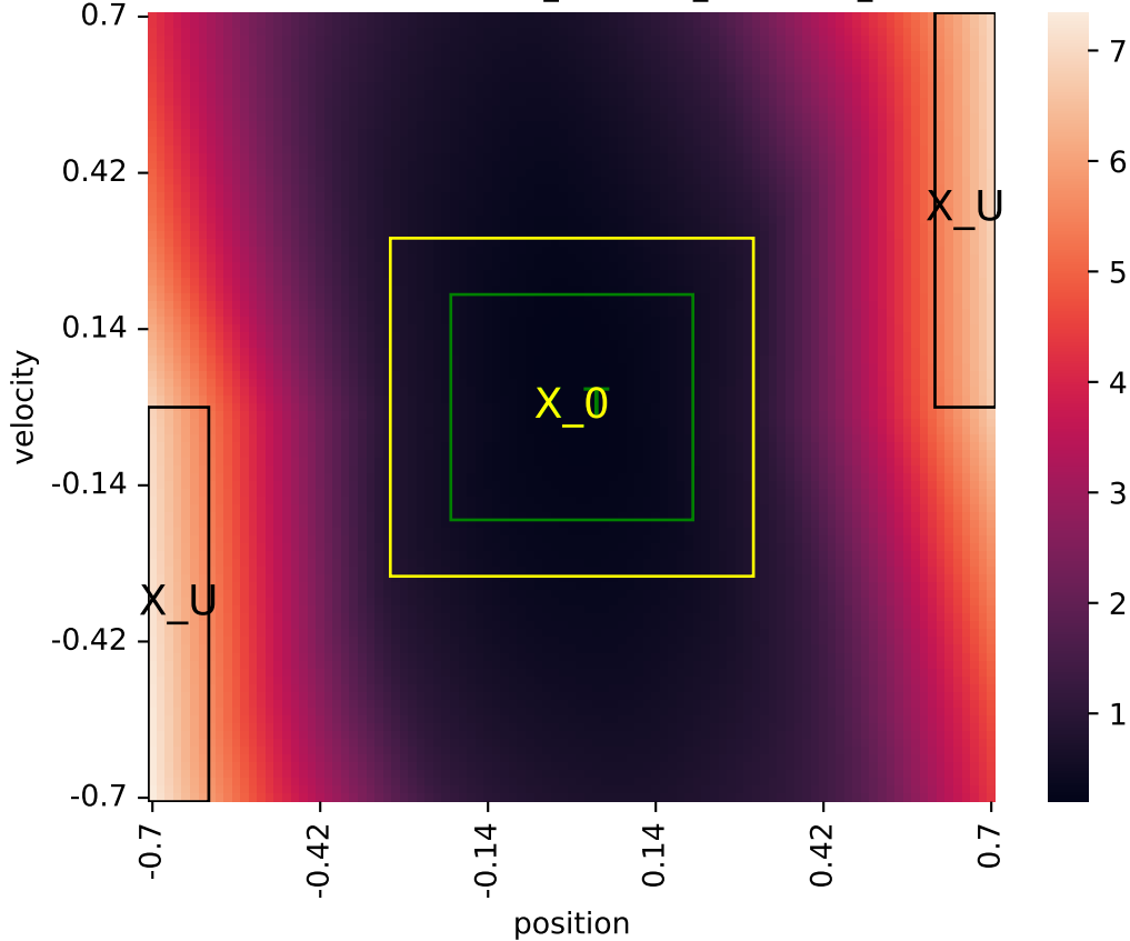
Learned certificate (2026-06-02_20-00-28_certificate_iteration=10)
