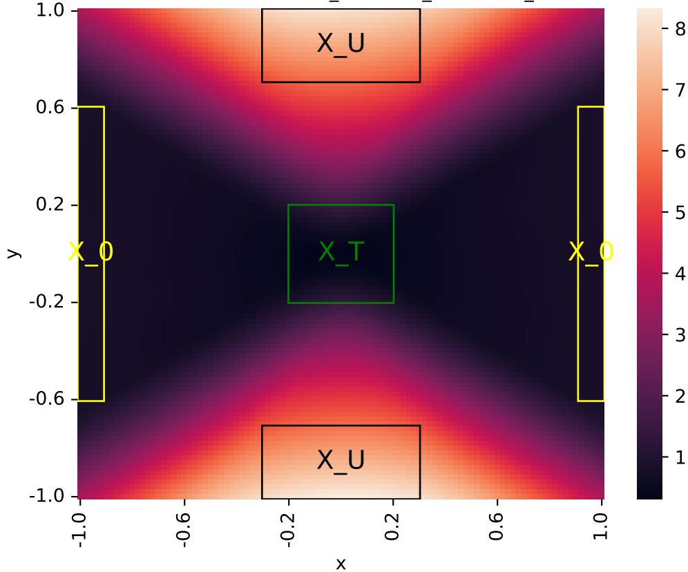
Learned certificate (2026-06-02_20-19-03_certificate_iteration=4)
