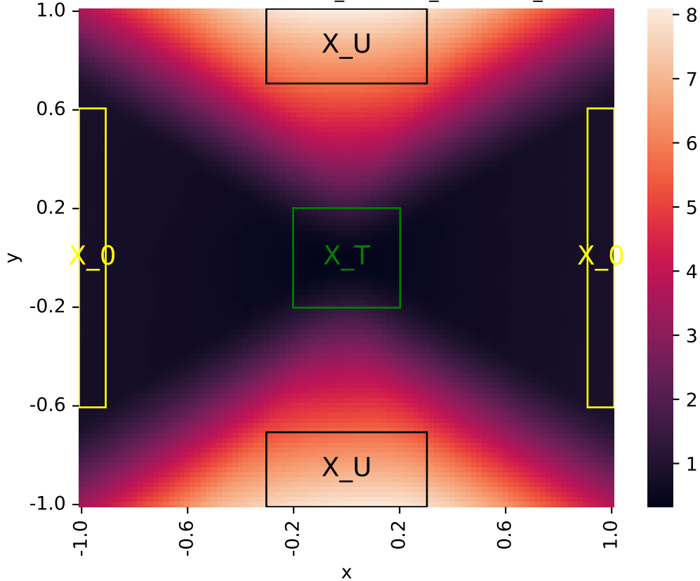
Learned certificate (2026-06-02_20-27-16_certificate_iteration=5)
