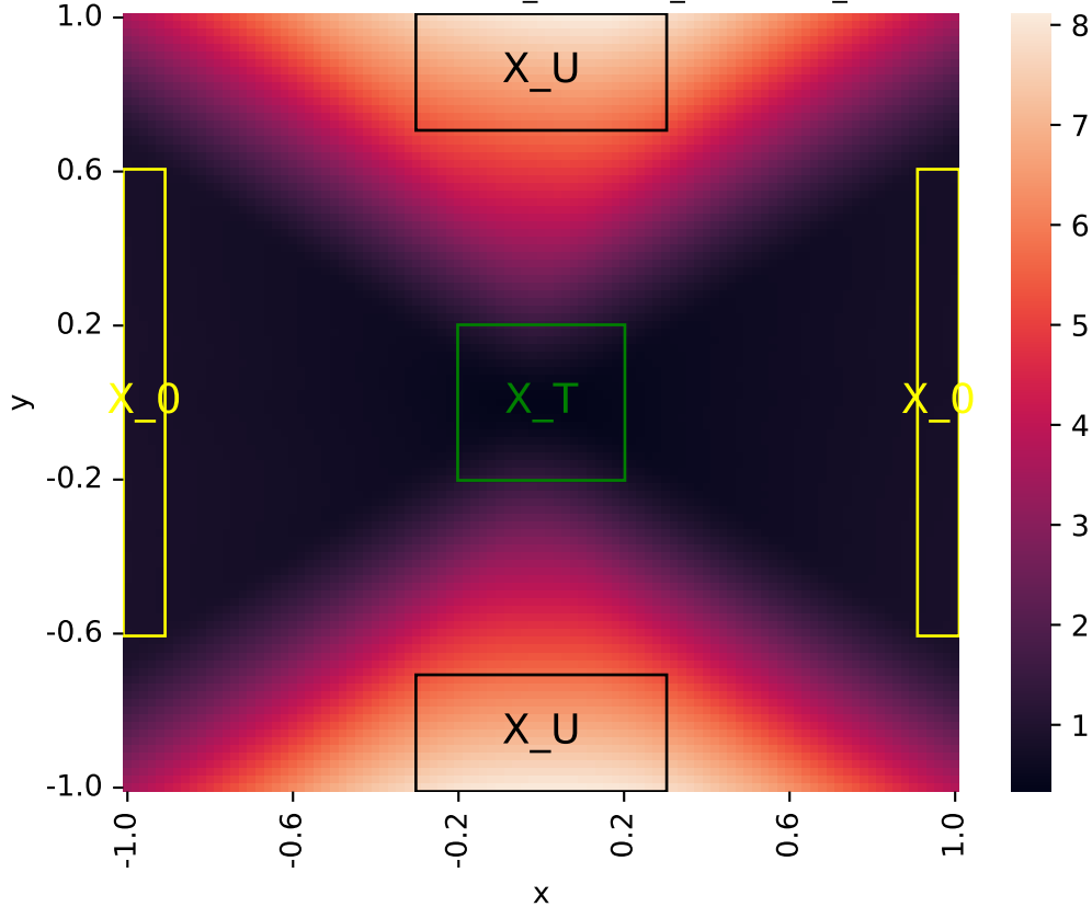
Learned certificate (2026-06-02_21-14-32_certificate_iteration=4)
