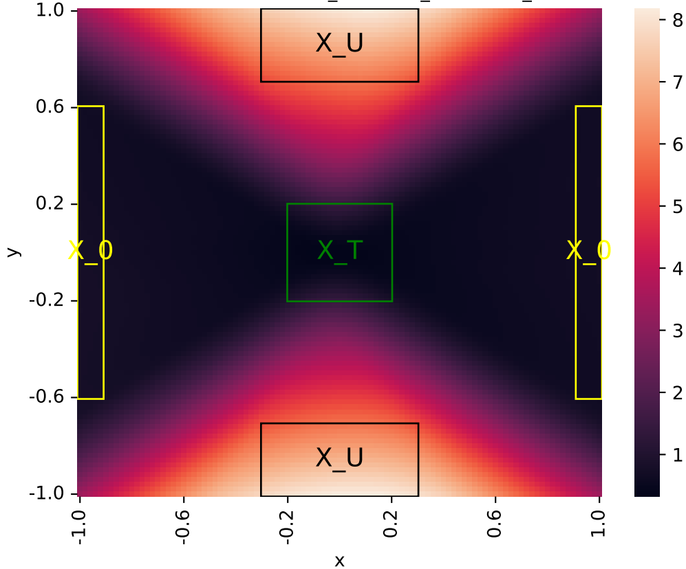
Learned certificate (2026-06-02_21-21-40_certificate_iteration=6)
