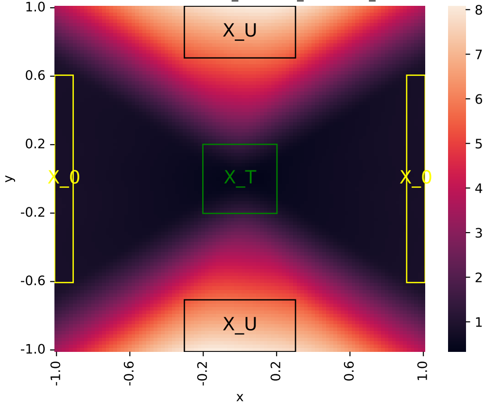
Learned certificate (2026-06-02_21-38-57_certificate_iteration=4)
