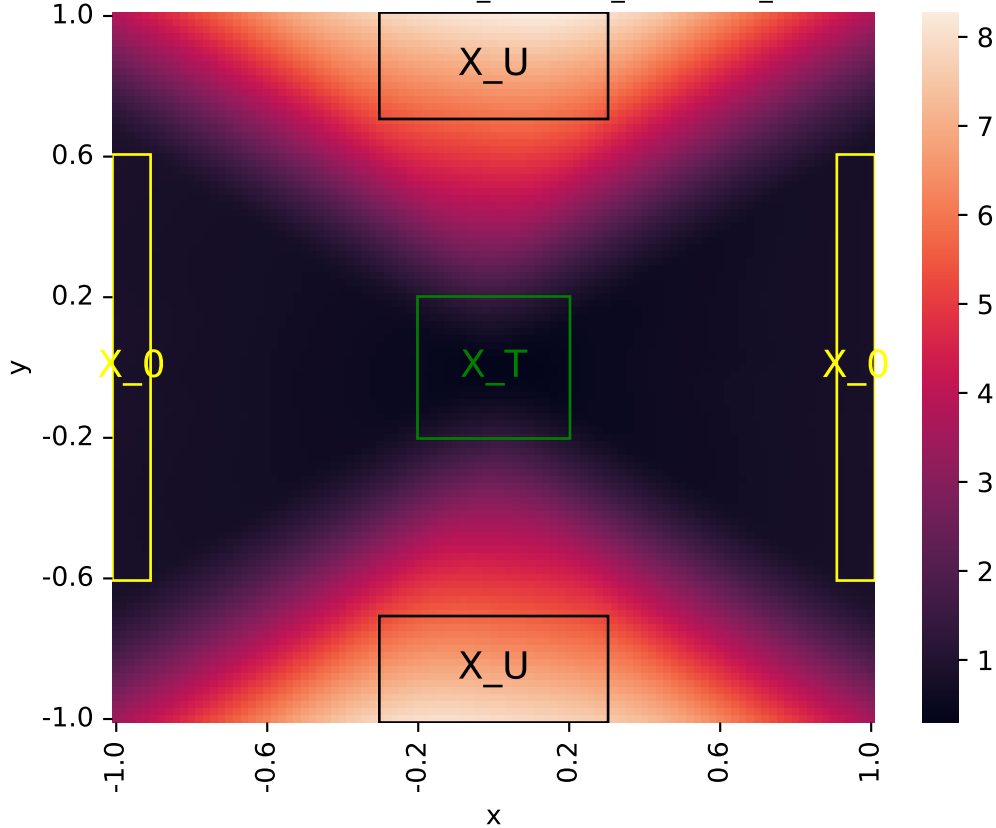
Learned certificate (2026-06-02_21-54-03_certificate_iteration=4)
