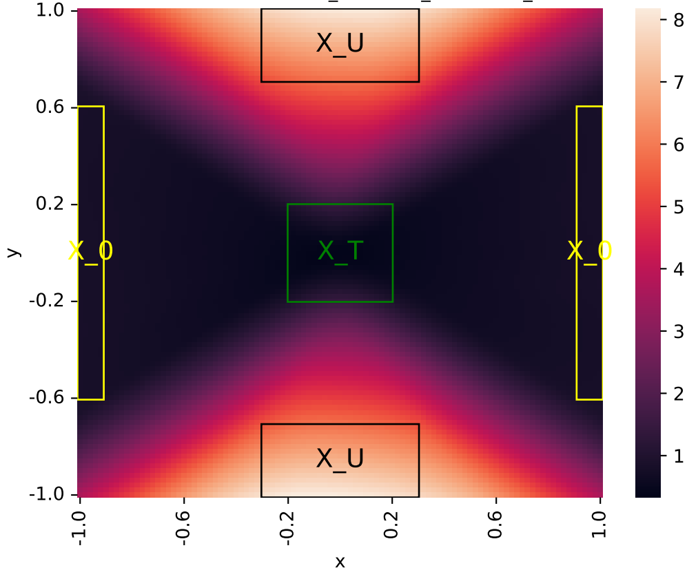
Learned certificate (2026-06-02_22-12-14_certificate_iteration=4)
