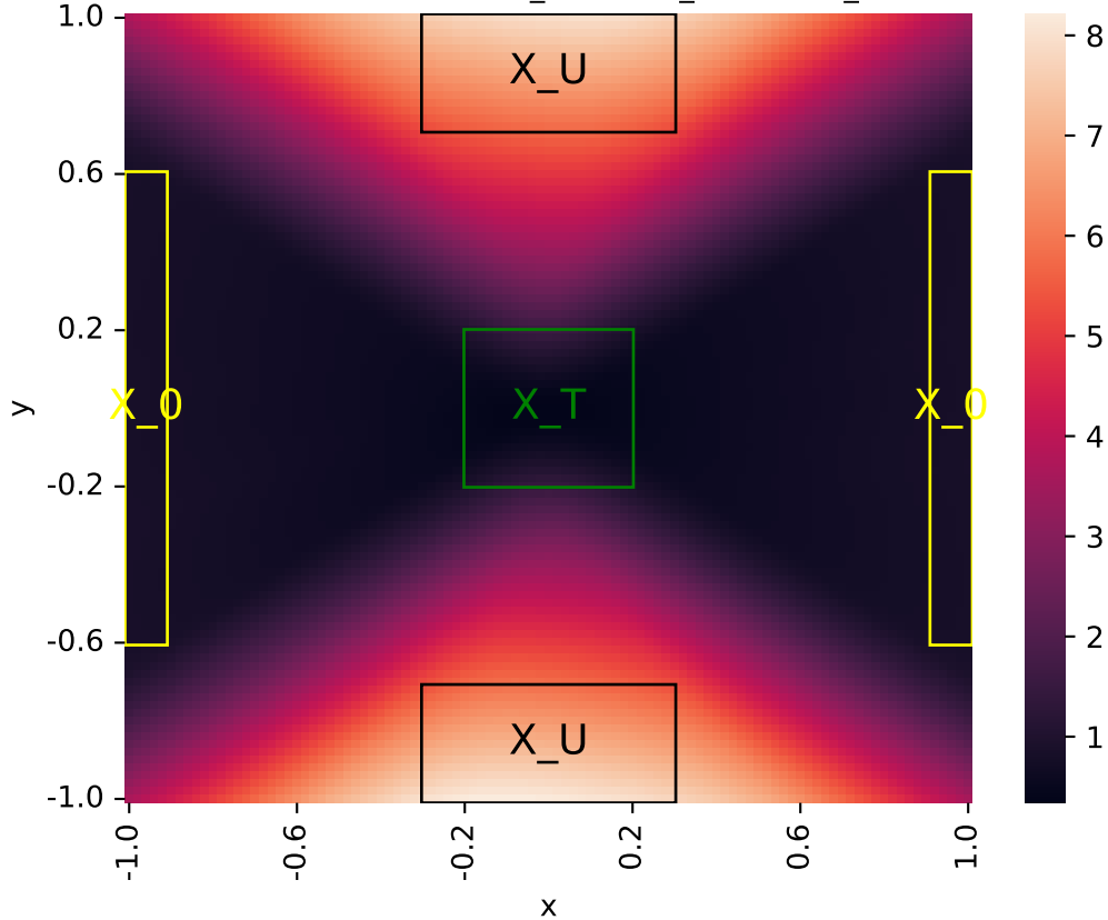
Learned certificate (2026-06-02_22-30-34_certificate_iteration=4)
