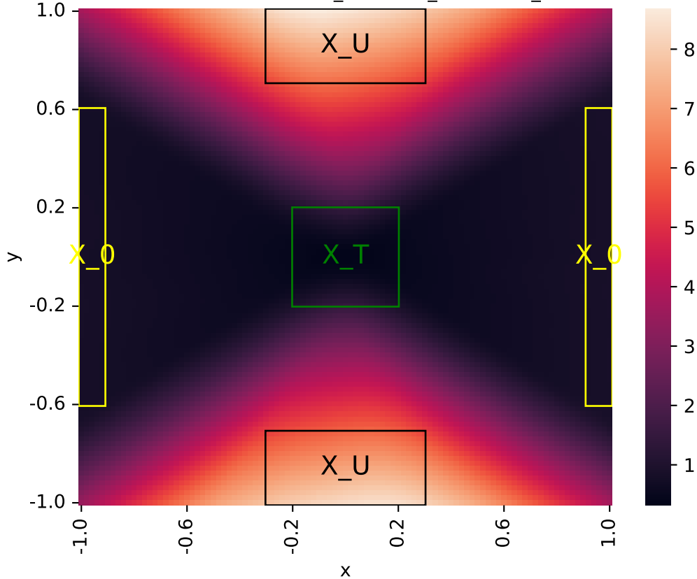
Learned certificate (2026-06-02_22-34-16_certificate_iteration=4)
