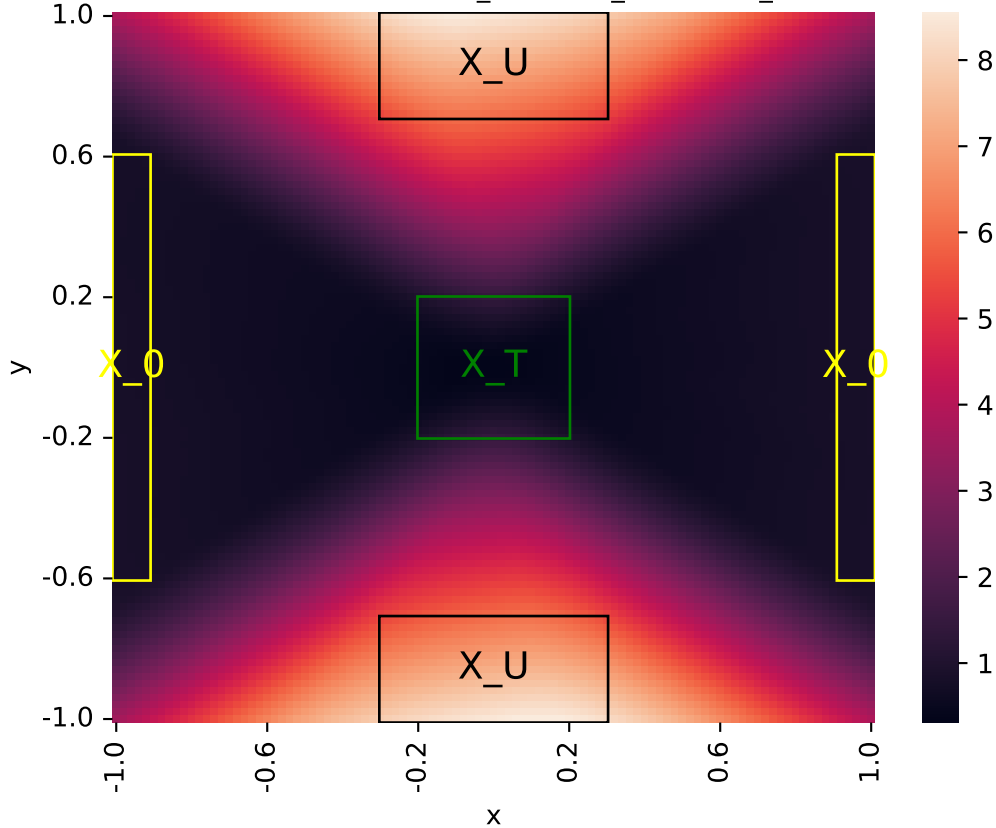
Learned certificate (2026-06-02_22-47-29_certificate_iteration=4)
