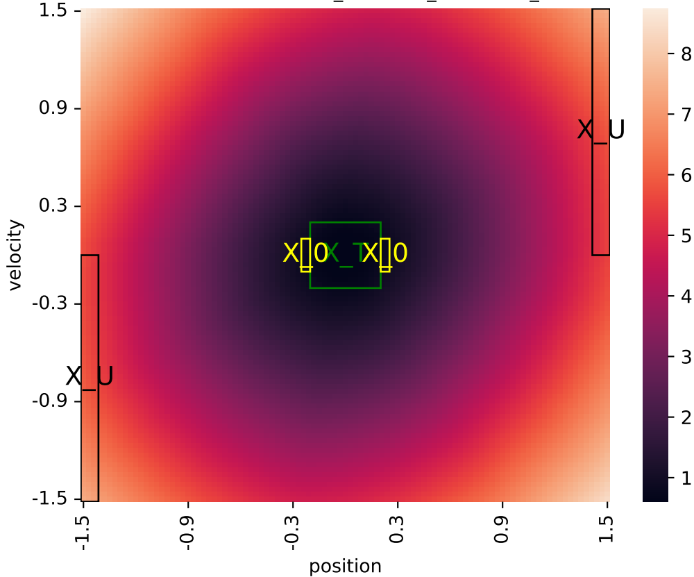
Learned certificate (2026-06-02_23-04-08_certificate_iteration=1)
