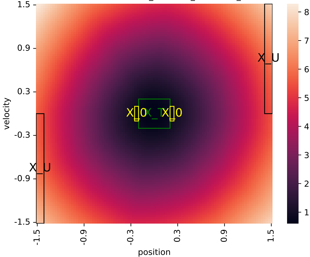
Learned certificate (2026-06-02_23-24-02_certificate_iteration=1)
