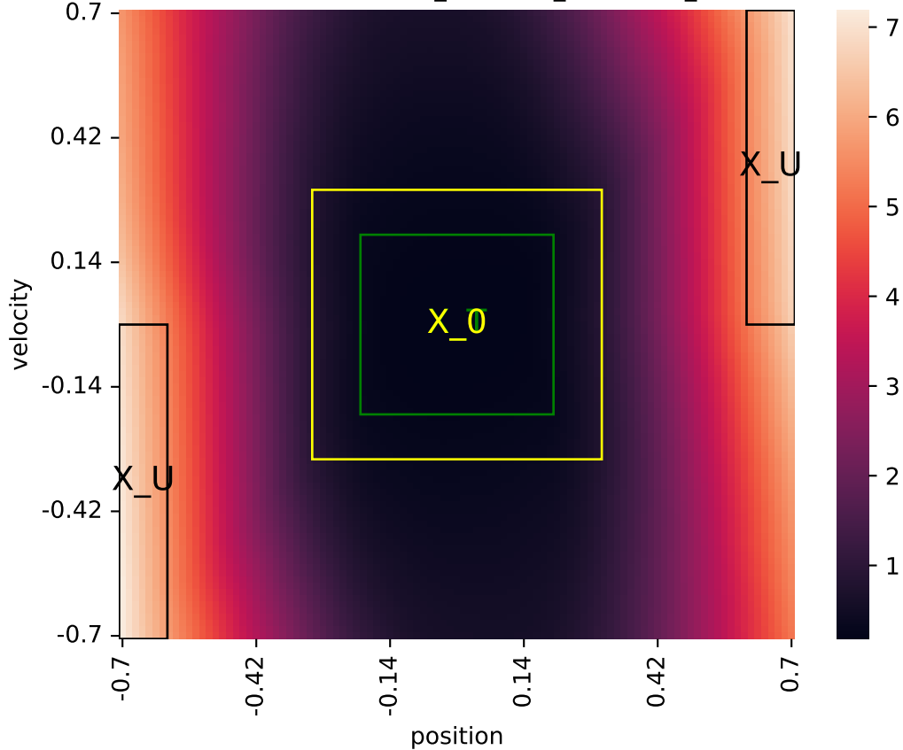
Learned certificate (2026-06-01_02-25-15_certificate_iteration=11)
