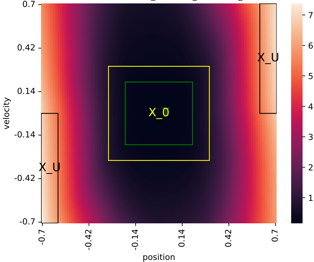
Learned certificate (2026-06-01_03-12-13_certificate_iteration=13)
