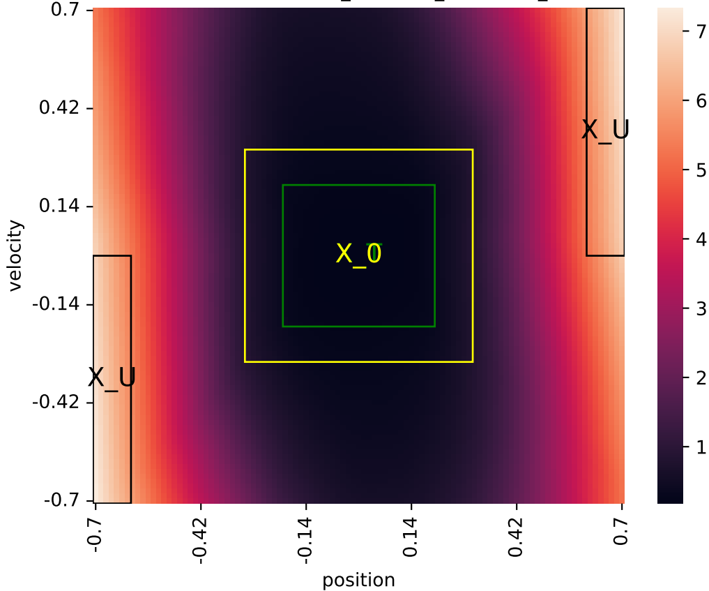
Learned certificate (2026-06-01_03-31-36_certificate_iteration=12)
