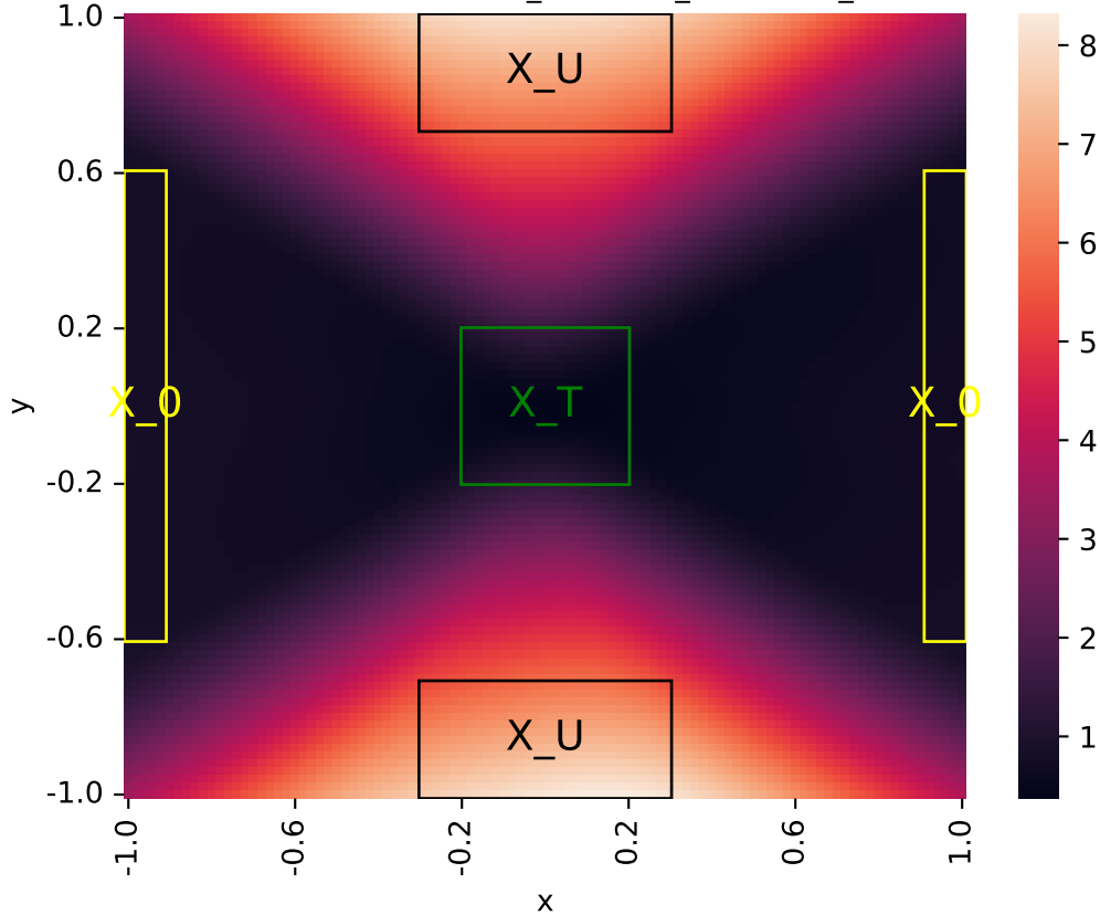
Learned certificate (2026-06-01_03-38-11_certificate_iteration=5)
