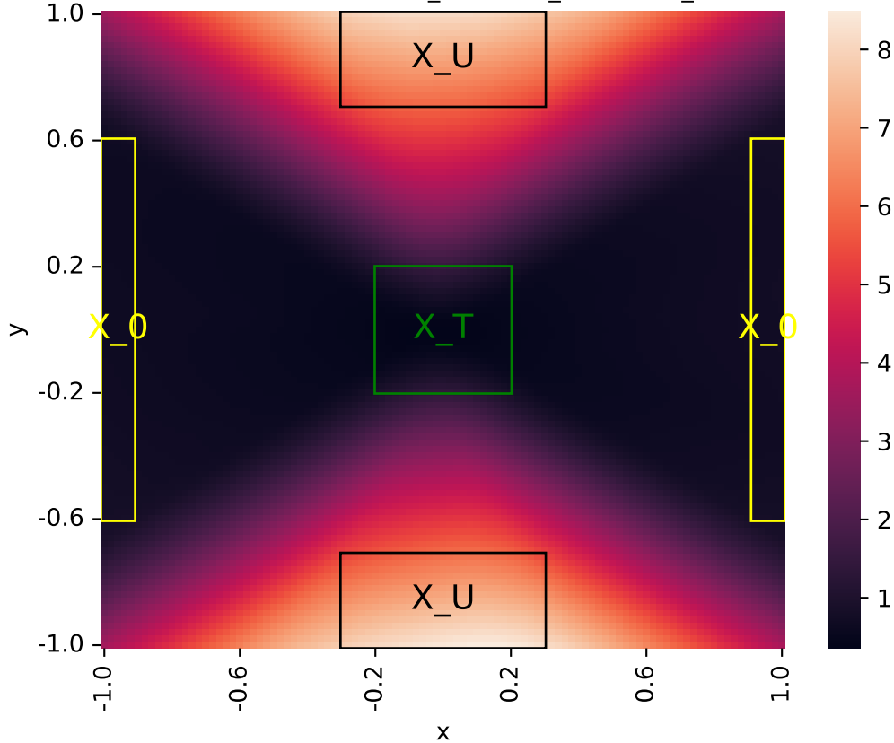
Learned certificate (2026-06-01_03-40-39_certificate_iteration=5)
