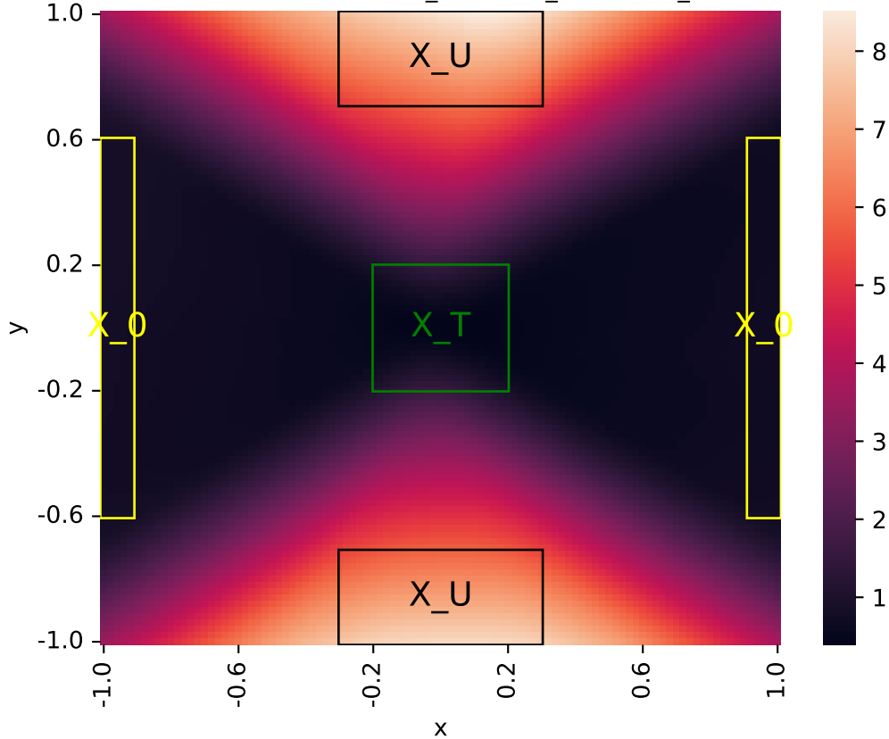
Learned certificate (2026-06-01_03-59-59_certificate_iteration=5)
