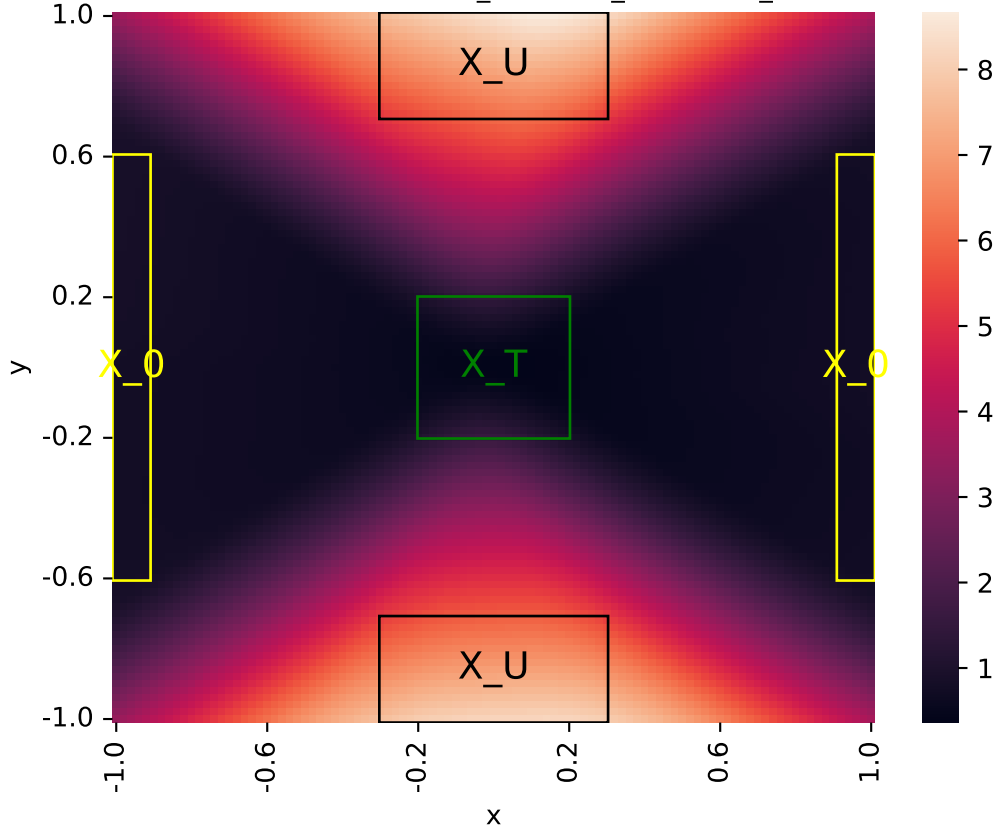
Learned certificate (2026-06-01_04-07-08_certificate_iteration=5)
