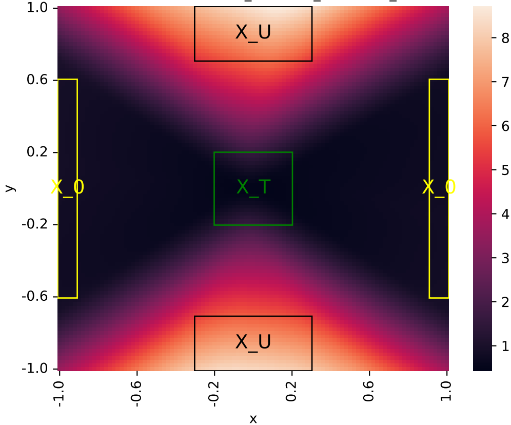
Learned certificate (2026-06-01_04-09-15_certificate_iteration=5)
