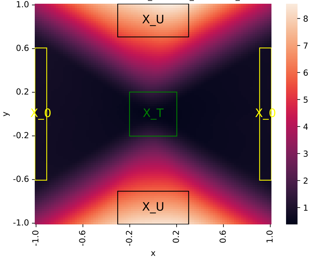
Learned certificate (2026-06-01_04-11-32_certificate_iteration=5)
