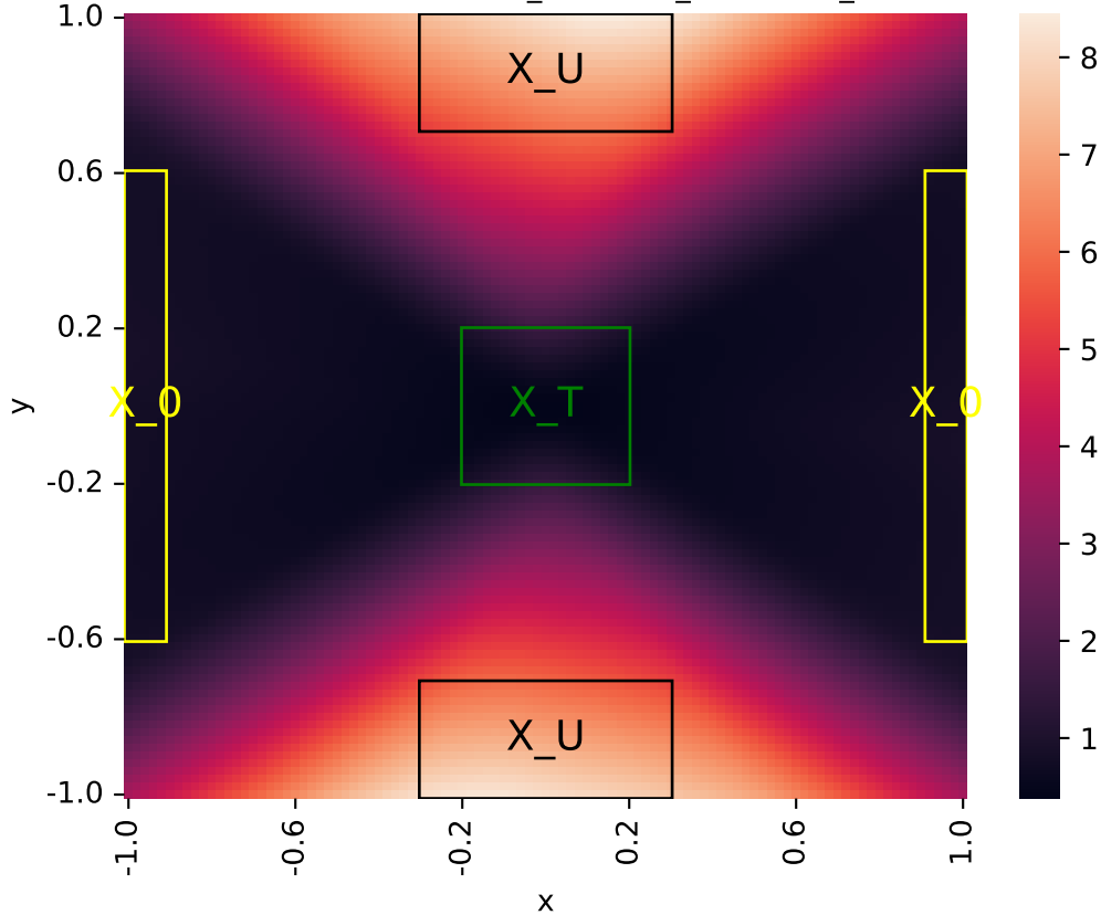
Learned certificate (2026-06-01_04-21-03_certificate_iteration=5)
