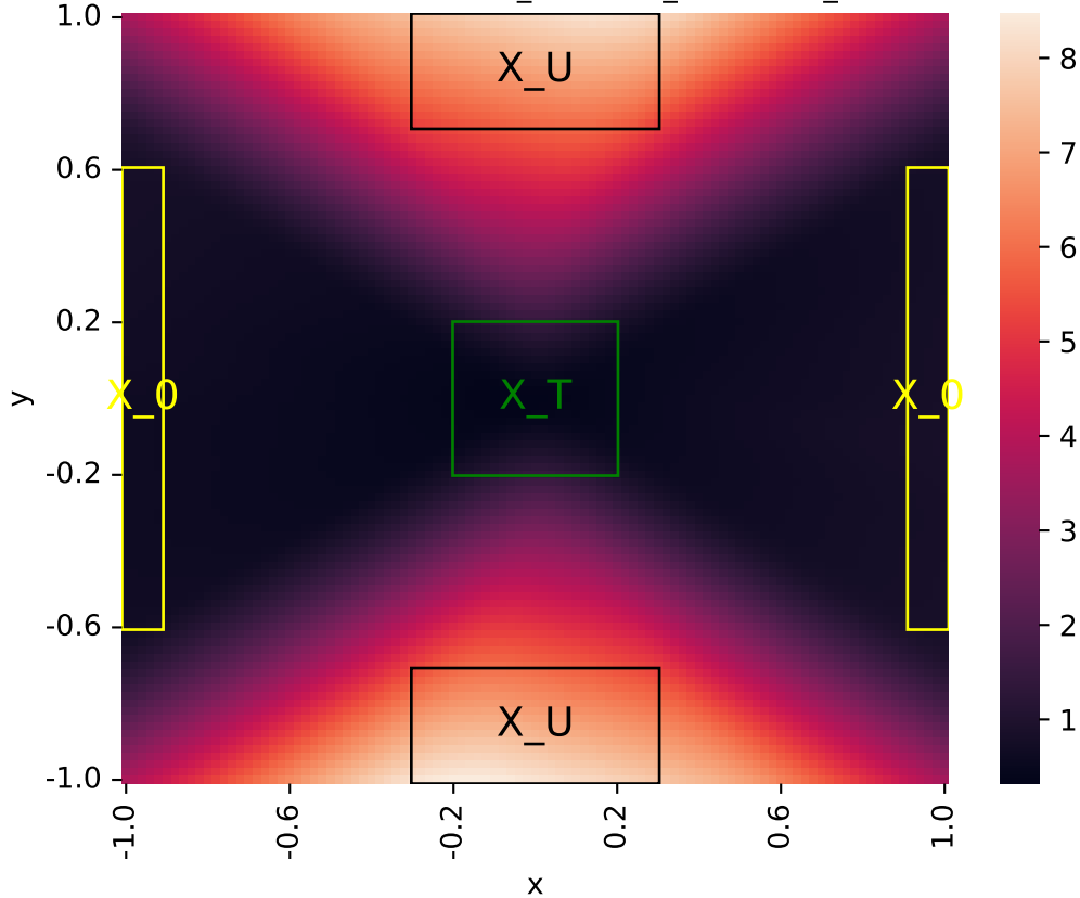
Learned certificate (2026-06-01_04-33-41_certificate_iteration=5)
