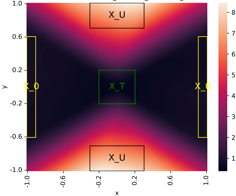
Learned certificate (2026-06-01_04-37-58_certificate_iteration=5)
