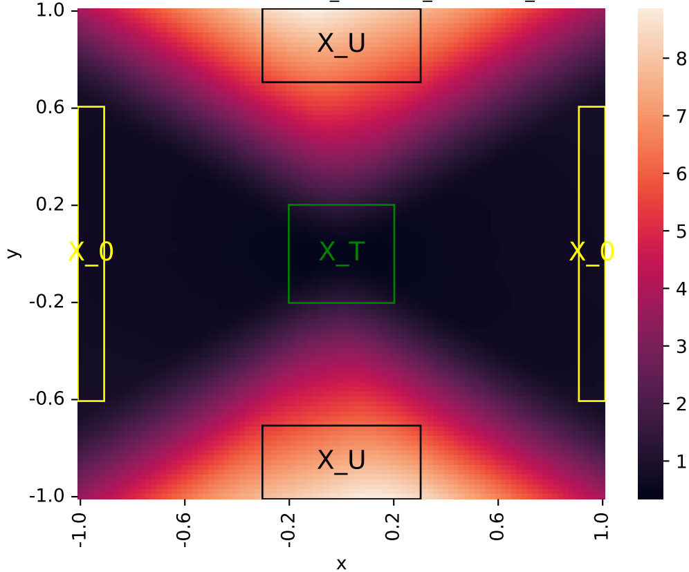
Learned certificate (2026-06-01_05-12-03_certificate_iteration=5)
