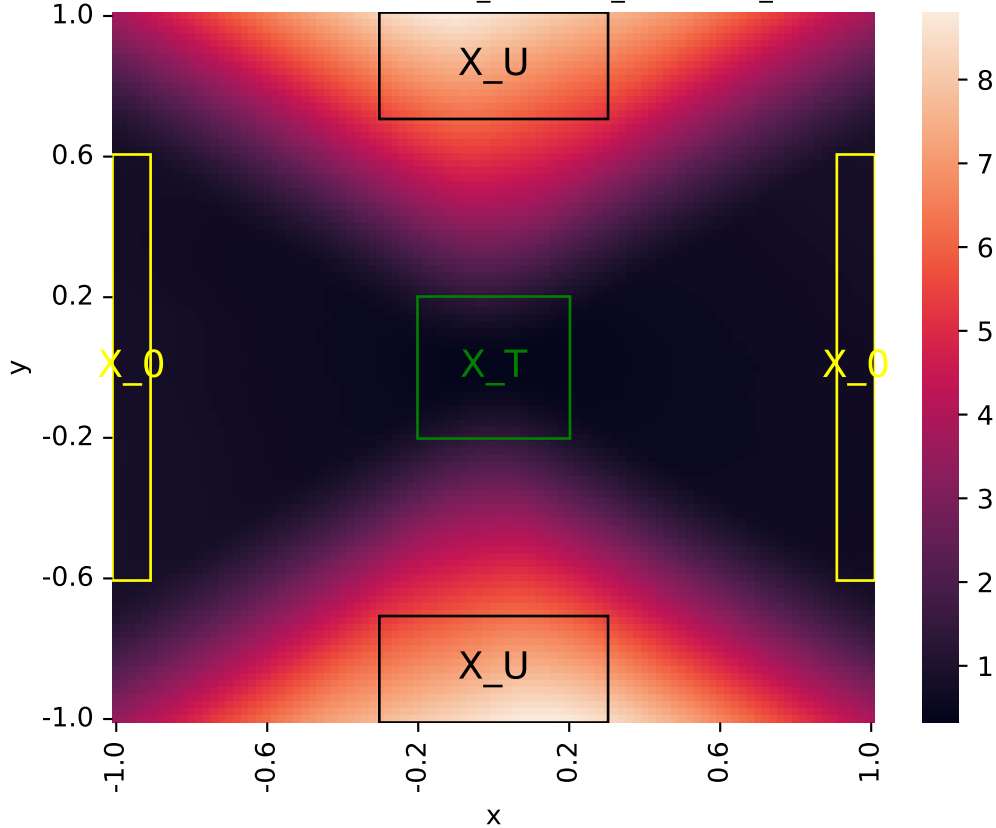
Learned certificate (2026-06-01_05-20-19_certificate_iteration=5)
