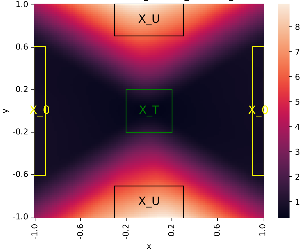
Learned certificate (2026-06-01_05-22-29_certificate_iteration=5)
